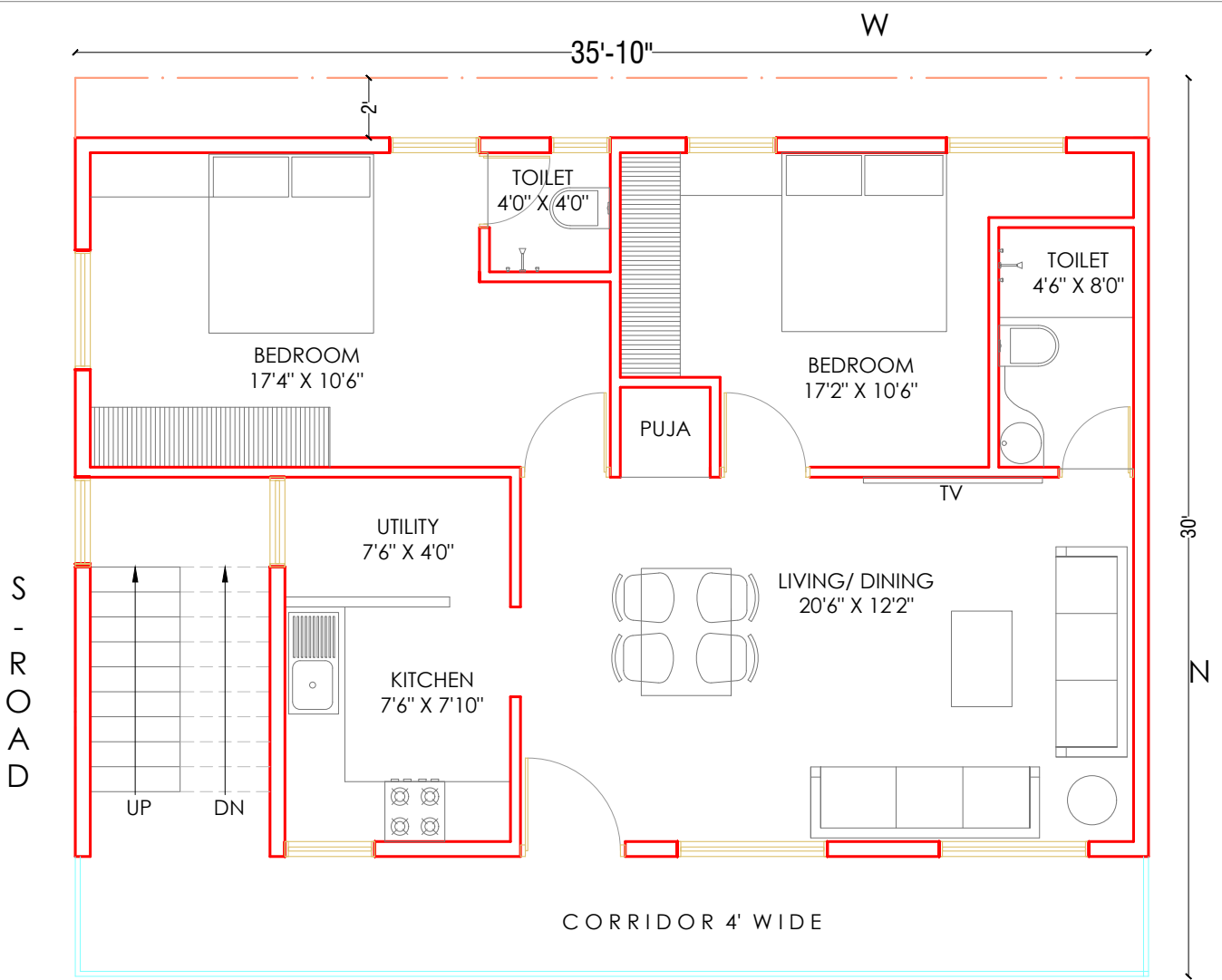
FIRST FLOOR PLAN BUILTUP :- 860 SFT CORRIDOR:- 145 SFT
